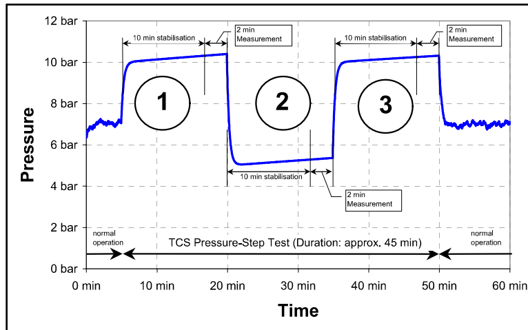
Principle of Pressure-Step-Method
