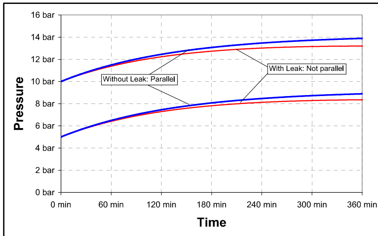
Evaluation of Pressure-Step-Method
