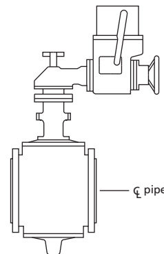
Style "B": Actuator mounted at right angle to pipe line.
